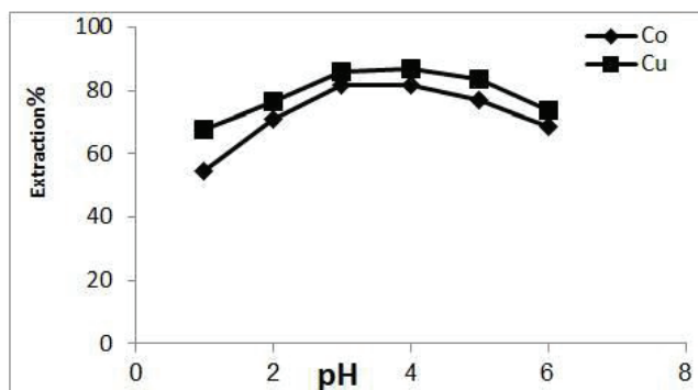
Fig. 2: PH effect on the determination of Cu (II) and Co (II) Conditions: Co (II) = 2.5 \mu g mL^{-1} , 15-C-5 = 1 \times 10^{-2} M , 0.4 mL of 2 % (v/v) Triton X-114 (b) Cu(II)-15-C-5 complex, Cu (II) = 2.5 \mu g mL^{-1} , 15-C-5 = 9 \times 10^{-3} M , 0.5 mL of 2 % (v/v) Triton X-114.
