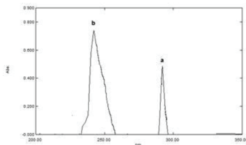
Fig. 1: Absorption spectra (a) Co(II)-15-C-5 complex, Co (II) = 2.5 \mu\text{g mL}^{-1} , 15-C-5 = 1 \times 10^{-2} M, pH = 4, 0.4 mL of 2 % (v/v) Triton X-114 (b) Cu(II)-15-C-5 complex, Cu (II) = 2.5 \mu\text{g mL}^{-1} , 15-C-5 = 9 \times 10^{-3} M, pH = 4, 0.5 mL of 2 % (v/v) Triton X-114.
